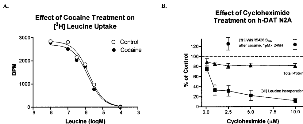
Fig. 10. A, Effects of (–)cocaine treatment (1 \mu M for 24 h) on [ ^3 H]leucine uptake in hDAT-N2A cells, from one of three independent experiments. Eight concentrations of [ ^3 H]leucine were used in each experiment, and the data were fit to a one-site model. There was no significant effect of (–)cocaine on V_{max} or K_m value. B, effects of cycloheximide treatment on protein synthesis in hDAT-N2A cells. Three or four pairs of independent saturation experiments were performed at each cycloheximide dose. A range of cycloheximide doses markedly inhibited [ ^3 H]leucine protein incorporation and mildly decreased total protein, but none blocked cocaine-induced increases in [ ^3 H]WIN 35428 binding. Comparing vehicle-treated, cocaine-treated (1 \mu M \times 24 h), and cocaine + cycloheximide-treated cells at each cycloheximide doses: 2.5 \mu M dose: F = 6.854 , df = 2, 8 , p < 0.05 , by one-way ANOVA, Tukey's post hoc; cocaine versus vehicle, q = 4.970 ; p < 0.05 ; cocaine + cyclo versus vehicle, q = 5.132 ; 10.0 \mu M dose: F = 29.58 , df = 2, 7 , p < 0.01 , Tukey's post hoc; cocaine versus vehicle, q = 10.27 , p < 0.01 ; cocaine + cyclo, q = 7.932 ; p < 0.01 .
