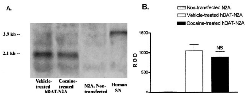
Fig. 9. A, digital image illustrating hDAT mRNA bands detected on electrophoretic gel: (–)cocaine treatment, 1 \mu M for 24 h; NT, N2A cells without hDAT transfection; SN, sample from human substantia nigra. B, graph depicting the results of three independent experiments. Gel results were digitized and the relative optical densities for each band quantitated and compared. There was no effect of cocaine treatment on hDAT mRNA band density (cocaine-treated versus control, t = 0.768 , df = 4 , p = 0.48 ).
