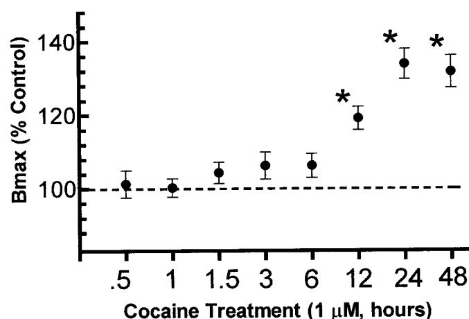
Fig. 2. Time course of cocaine effects on [ ^3 H]WIN 35428 B_{\max} in hDAT-N2A cells. Cells were grown to confluence, then treated with fresh medium containing either cocaine or the same volume of medium only. Cells were initially treated with cocaine, 10^{-6} M for the indicated time periods, from 0.5 to 48 h. Cells used in the 48-h experiment were washed after 24 h and supplied with fresh cocaine or vehicle. Eight concentrations of [ ^3 H]WIN 35428 were used in each experiment, and the data fit to a one-site model. Three to five pairs of independent saturation experiments were performed at each time point, and the raw data was analyzed as matched pairs. A repeated-measures, two-way ANOVA found there were significant cocaine ( df = 15, 1 , F = 3.92 , p = 0.04 ) and time effects ( df = 15, 7 , F = 33.3 , p < 0.001 ) on [ ^3 H]WIN 35428 B_{\max} . Follow-up paired t tests found there were significant cocaine effects at 12 ( t = 4.87 , p = 0.02 ), 24 ( t = 6.83 , p = 0.02 ), and 48 h ( t = 5.15 , p = 0.05 ). There were no effects on binding affinity.
