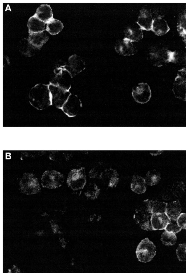
Fig. 6. Digital image displaying hDAT immunofluorescence pattern detected in hDAT-N2A cells using confocal microscopy. A, after (-)cocaine treatment, 1 \mu\text{M} for 24 h. B, after vehicle treatment. Compared with vehicle, a number of cells demonstrate more intense labeling of the outer membrane (as viewed at 200\times ), and less internal DAT immunofluorescence. The intensity of fluorescence rather than area was measured. The entire plasma membrane was outlined at each level, including bright and less intense regions for each cell, by a technician who was blind to treatment condition. For cells that were confluent, the region of interest outlined was divided midway through the section that seemed joined.
