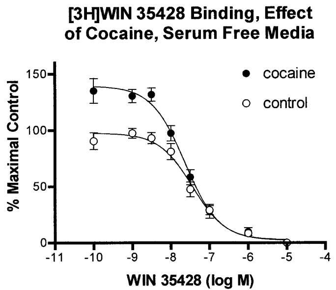
Fig. 12. Effect of (–) cocaine treatment (1 \mu M, 24 h) on [ ^3 H]WIN 35428 binding similarly in serum-free medium. Homologous displacement curves above (above data averaged from three pairs of independent experiments) demonstrated a similar increase after cocaine treatment as found in cells grown in FBS containing medium. The [ ^3 H]WIN 35428 B_{max} was increased 29 \pm 6\% versus paired controls, but K_d was unchanged.
