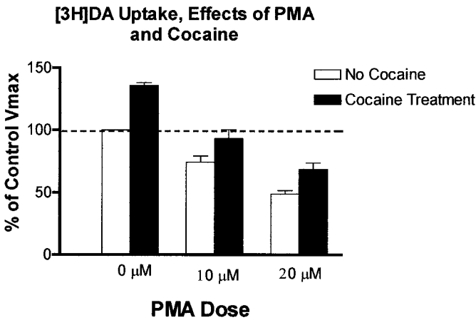
Fig. 11. Effects of both (–)cocaine and PMA treatment: the cocaine treatment was performed as described in other experiments. hDAT-N2A cells were treated with PMA for 15 min at final concentrations of 0, 10, and 20 \mu M before uptake assay. Both treatments had the expected effects without any apparent interference.
