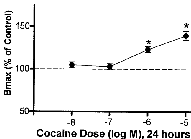
Fig. 1. Effects of (–)-cocaine on [ ^3 H]WIN 35428 binding to hDAT-N2A cells. Cells were grown to confluence, then treated for 24 h with fresh medium containing either (–)-cocaine ( 10^{-8} M to 10^{-5} M) or the same volume of medium only. n = 5 pairs of independent saturation experiments for each (–)-cocaine concentration. Eight concentrations of [ ^3 H]WIN 35428 were used in each experiment, and the data fit to a one-site model. At higher doses, 10^{-6} and 10^{-5} M, cocaine significantly increased [ ^3 H]WIN 35428 binding sites (one-way ANOVA, df = 4, 23 , F = 15.27 , p < 0.0001 , 10^{-5} M different from control, Tukey's post hoc q = 9.79 , p < 0.001 , 10^{-6} M different from control, Tukey's post hoc q = 5.05 , p < 0.05 ). There were no effects on binding affinity.
